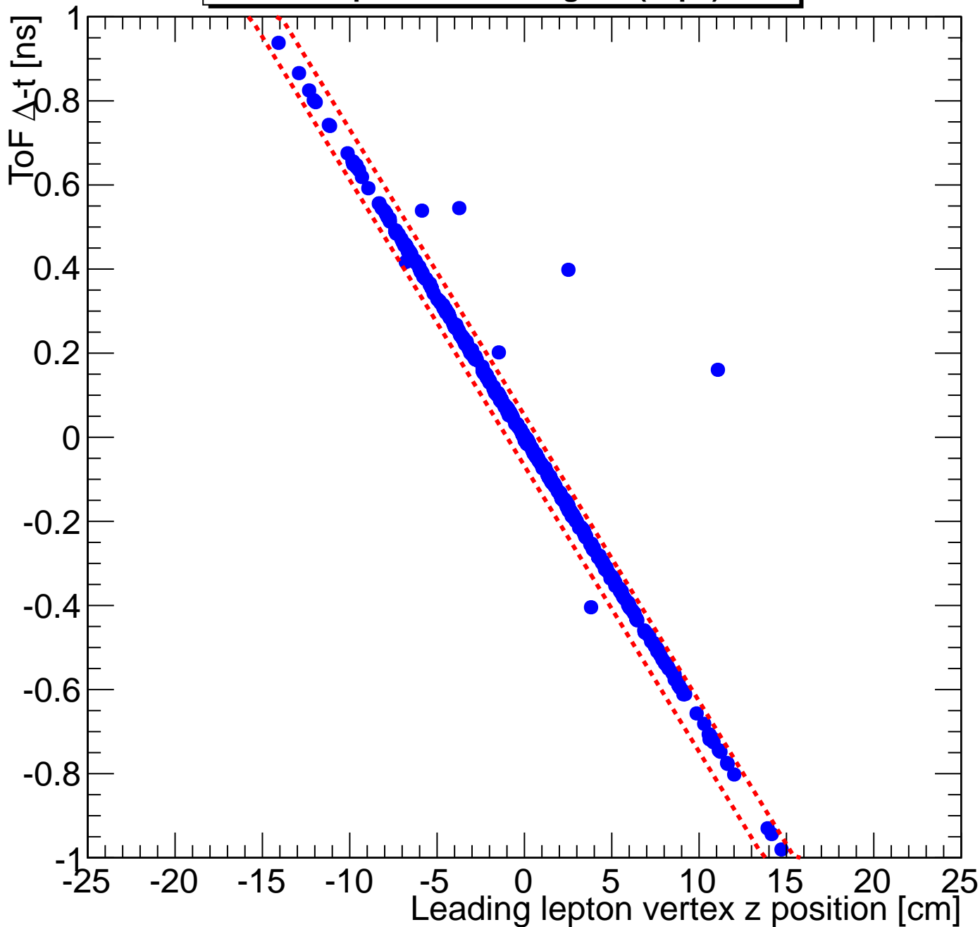
Both protons from signal (10ps)
