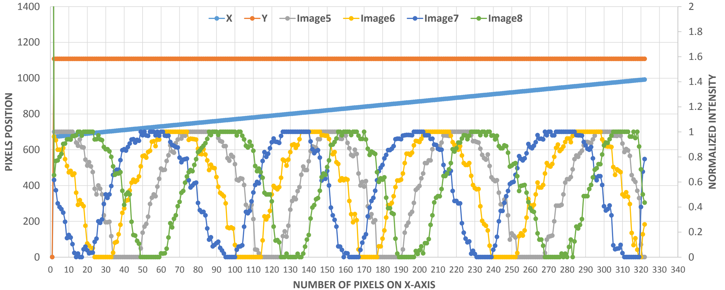
Phase shift of the fringes at single pixel horizontal line at last 4 images
